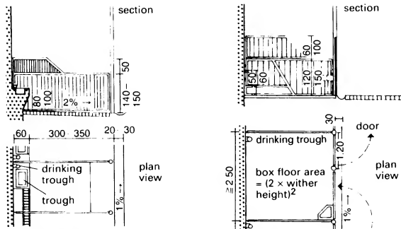
2 Tethered stall arranged as box stall
